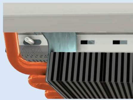
SLOT ADJUSTMENT 2
