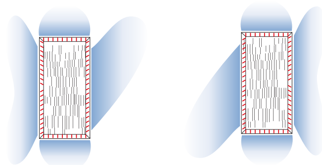
An example of the LYRA II in a high airflow application at a symmetrical setting, where flow pattern control blades are set a 30° angle to avoid the colliding air streams from opposing chilled beam units. This throw pattern is unique to the LYRA II.
